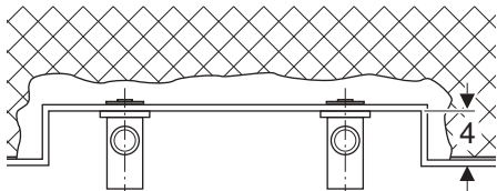
Figure 196: Installation dimension for concealed installation with a Geberit mounting plate, offset
