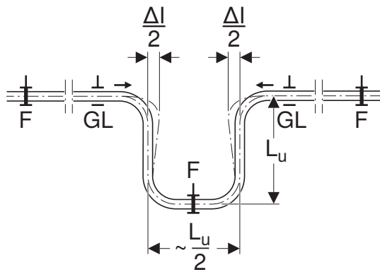
Figure 159: U-bend, made of bent pipe
