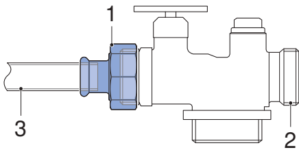
Figure 125: Connection to gas valves, conical-sealing
