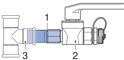
Figure 117: Connection to male thread
