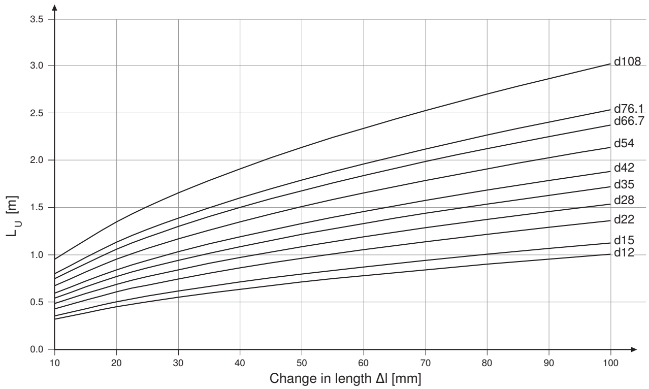
Figure 176: Deflection leg length L_U , copper pipes according to EN 1057
