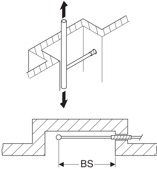
Figure 152: Straight deflection leg, without insulation
