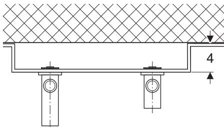
Figure 197: Installation dimension for exposed installation with a Geberit mounting plate, offset
