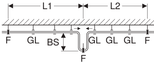
Figure 149: Expansion compensation by a U-bend
