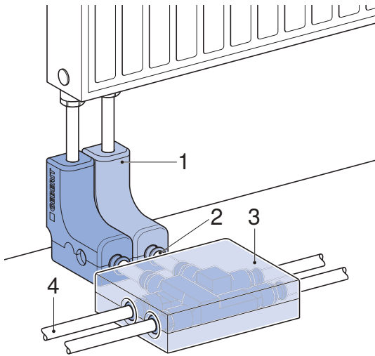
Figure 75: Radiator connection for pipe laying with a distance to the wall
