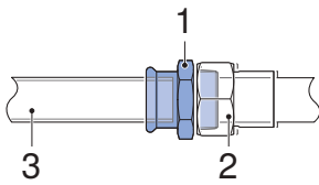
Figure 112: Connection to female thread
