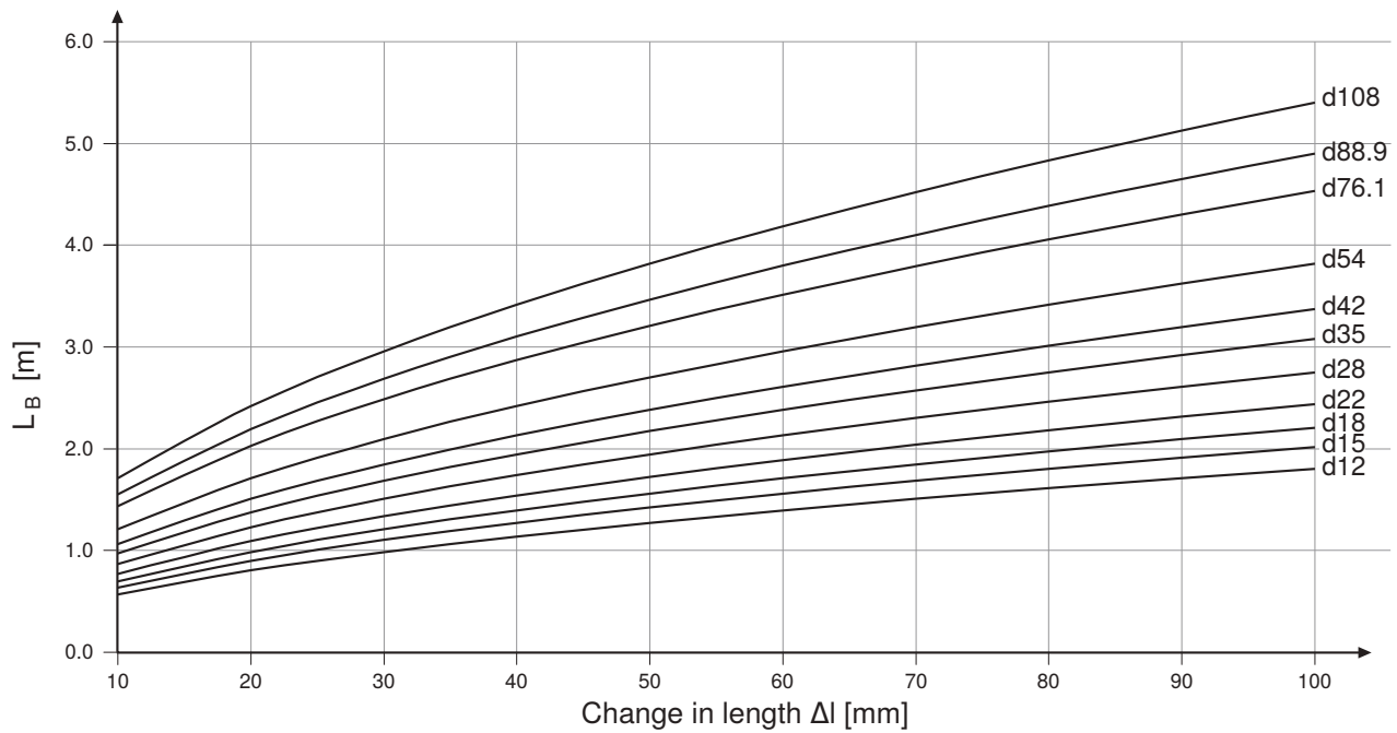
Figure 171: Deflection leg length L B , copper pipes according toDVGW GW 392:2015-04
