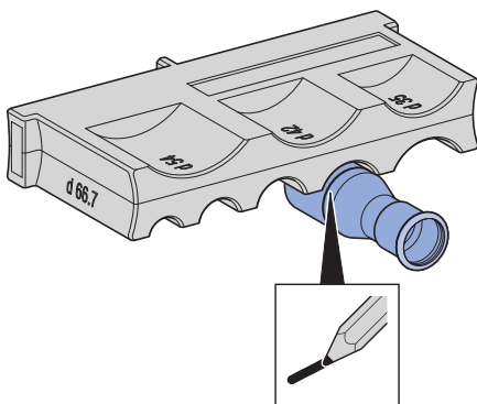
Figure 204: Marking of the insertion distance on fittings with a plain end
