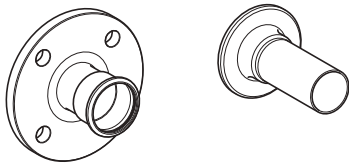
Figure 140: Flange connections
