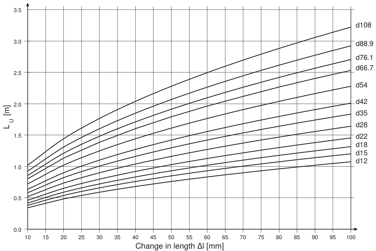
Figure 168: Deflection leg length L U , Geberit Mapress Carbon Steel
