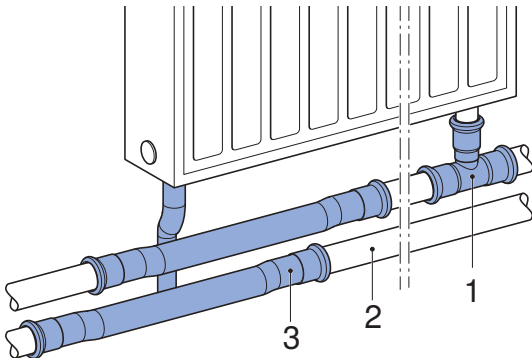
Figure 129: Connection for surface-mounted pipe (skirting board), with a distance between the inlet and return flow
