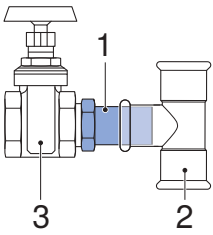
Figure 69: Connection to stop valve
