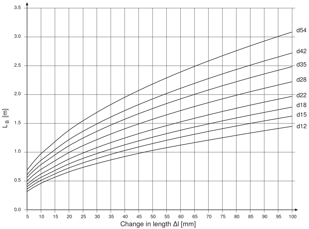
Figure 158: Deflection leg length L_B , stainless steel 1.4521
