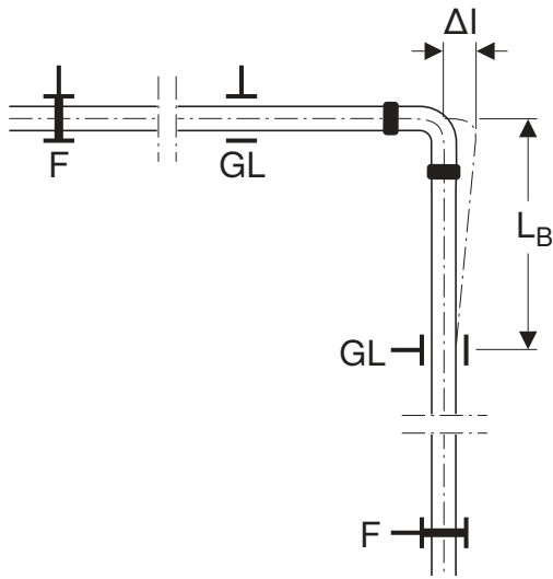
Figure 163: Expansion compensation with a change in direction
