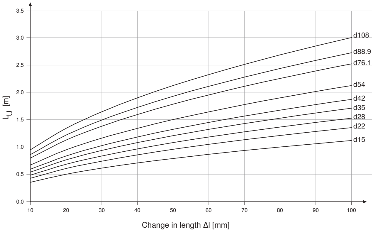
Figure 182: Deflection leg length L U , Geberit Mapress CuNiFe
