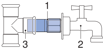
Figure 116: Connection to outside tap
