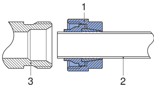
Figure 133: Union connector for Euro cone
