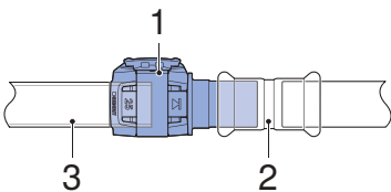
Figure 66: Connection to Geberit FlowFit
