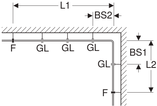
Figure 148: Expansion compensation through change in direction
