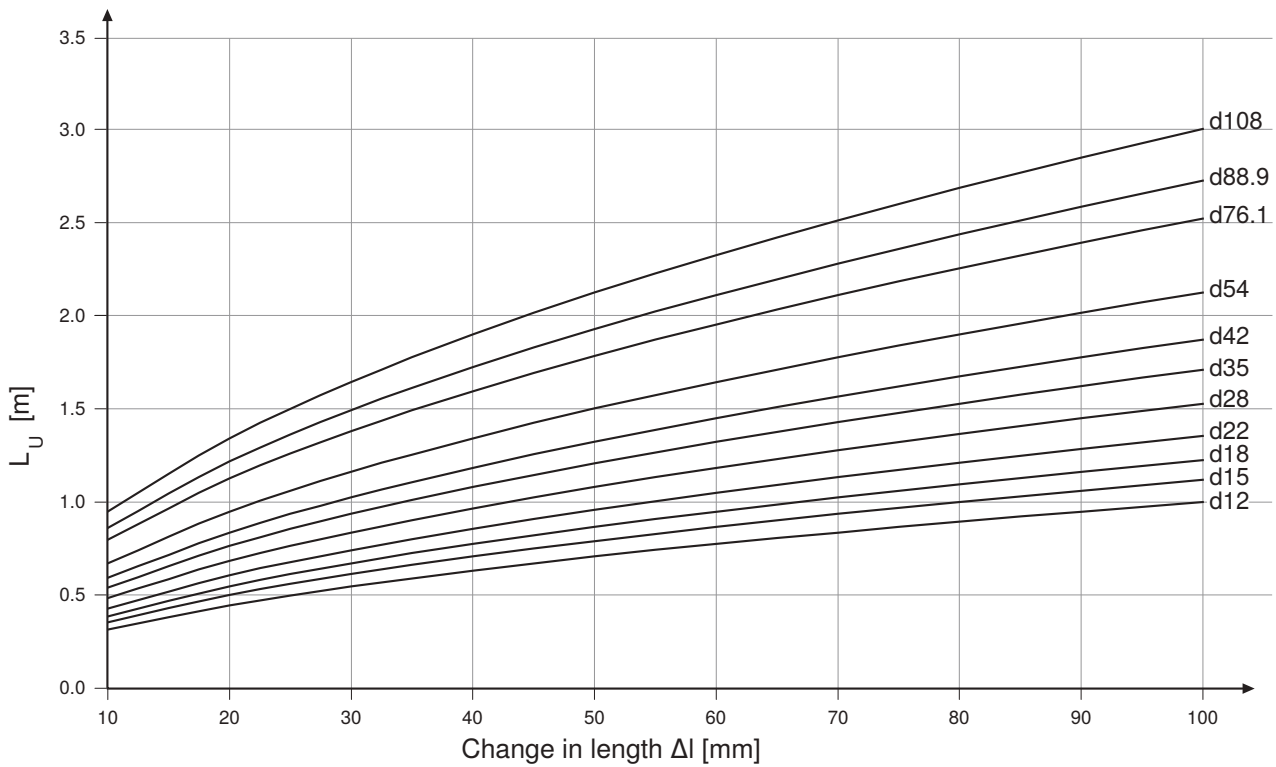
Figure 175: Deflection leg length L U , copper pipes according to DVGW GW 392:2015-04
