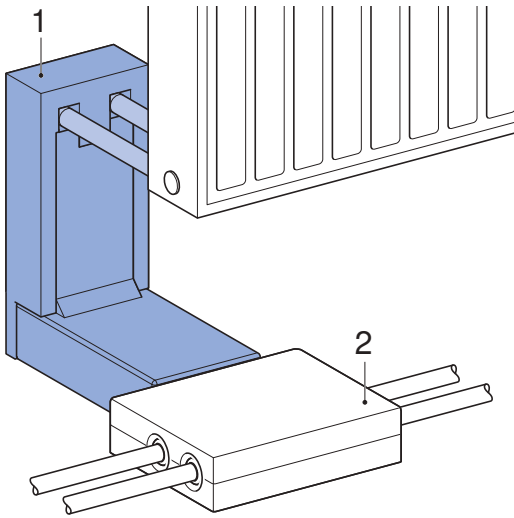
Figure 86: Radiator connector box type C for higher screed constructions
