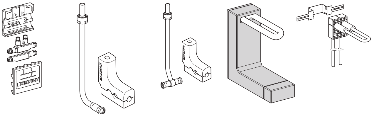
Figure 97: Geberit connections for heating
