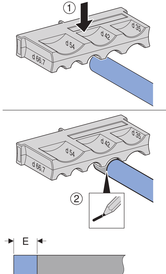
Figure 203: Marking of the insertion distance
