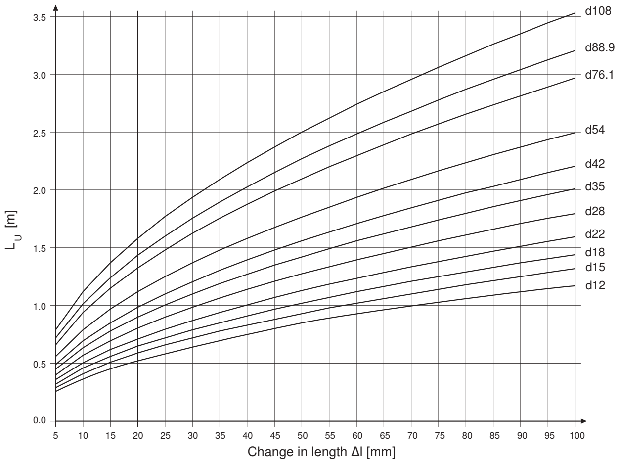
Figure 161: Deflection leg length L U , stainless steel 1.4401
