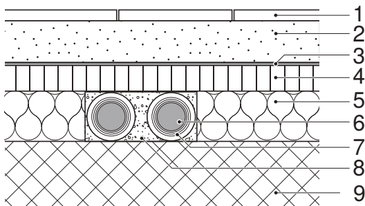
Figure 195: Pipe laying on uncovered concrete floors
