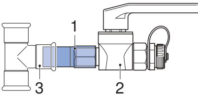
Figure 71: Connection to male thread
