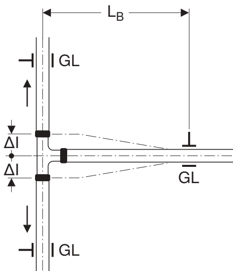
Figure 164: Expansion compensation with branch pipe
