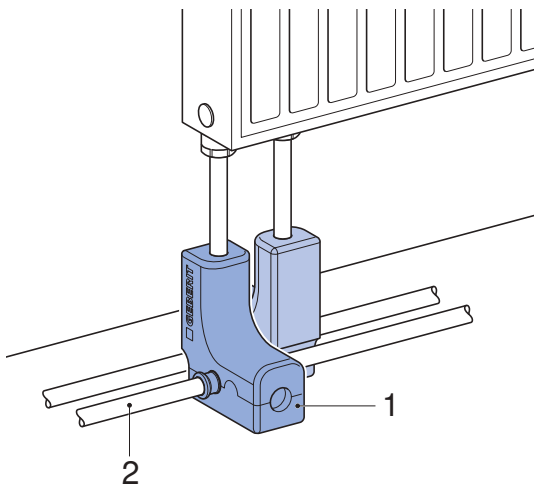
Figure 76: Radiator connection for pipe laying near the wall
