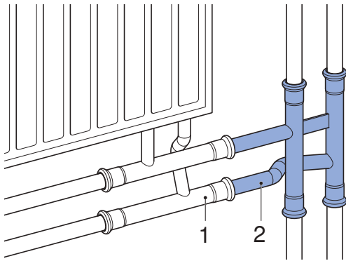
Figure 78: Connection to riser pipe, 1 radiators
