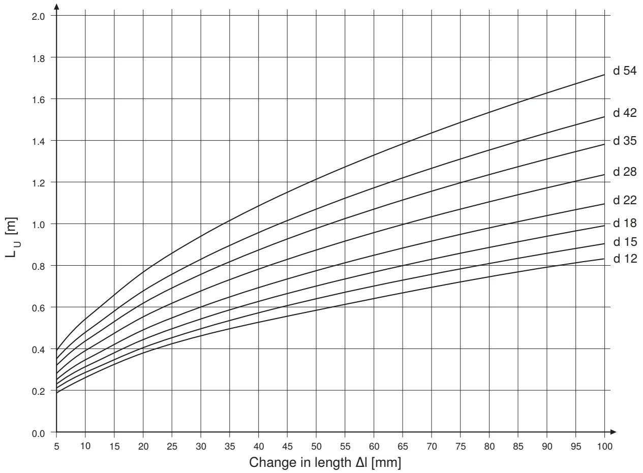
Figure 162: Deflection leg length L_u , stainless steel 1.4521
