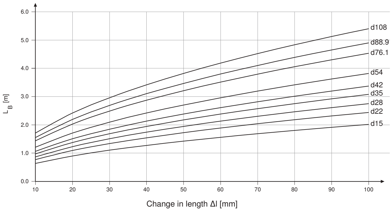
Figure 179: Deflection leg length L_B , Geberit Mapress CuNiFe
