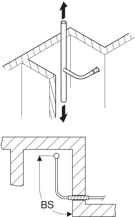
Figure 153: Bent deflection leg, without insulation
