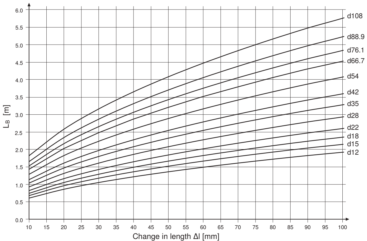
Figure 165: Deflection leg length L_B , Geberit Mapress Carbon Steel
