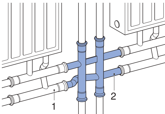
Figure 79: Connection to riser pipe, 2 radiators
