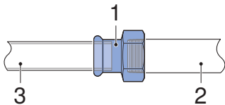
Figure 34: Connection to male thread
