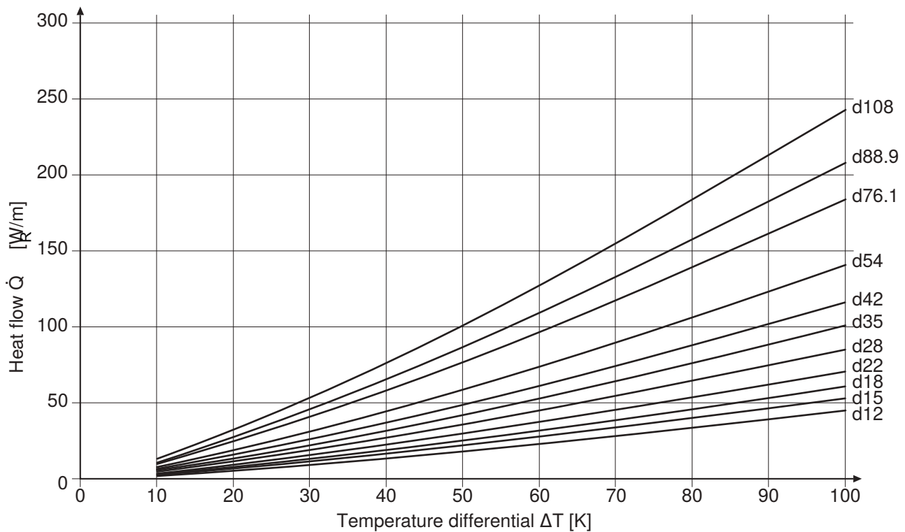
Figure 212: Heat emission for Geberit Mapress Carbon Steel system pipes
