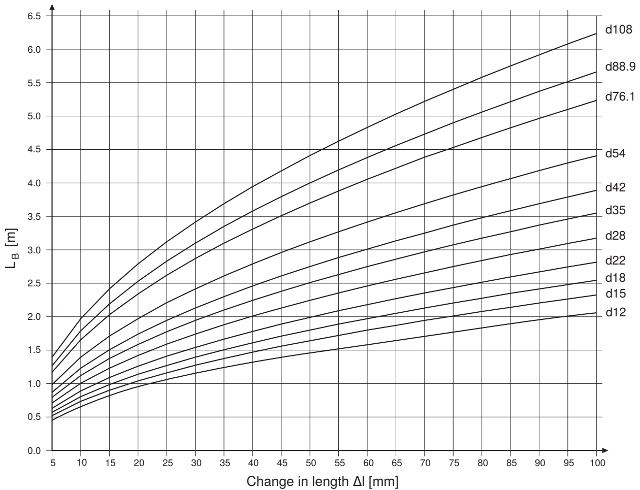
Figure 157: Deflection leg length L B , stainless steel 1.4401
