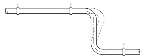
Figure 146: Absorption of a change in length \Delta l by the elasticity of the piping system
