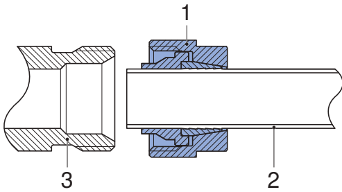
Figure 84: Union connector for Euro cone
