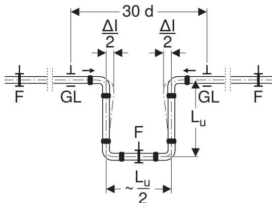
Figure 160: U-bend, made with pressfittings
