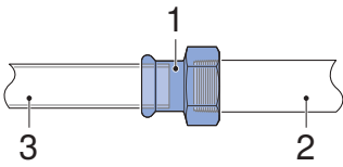
Figure 70: Connection to male thread
