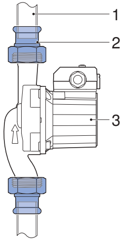
Figure 122: Connection to male thread
