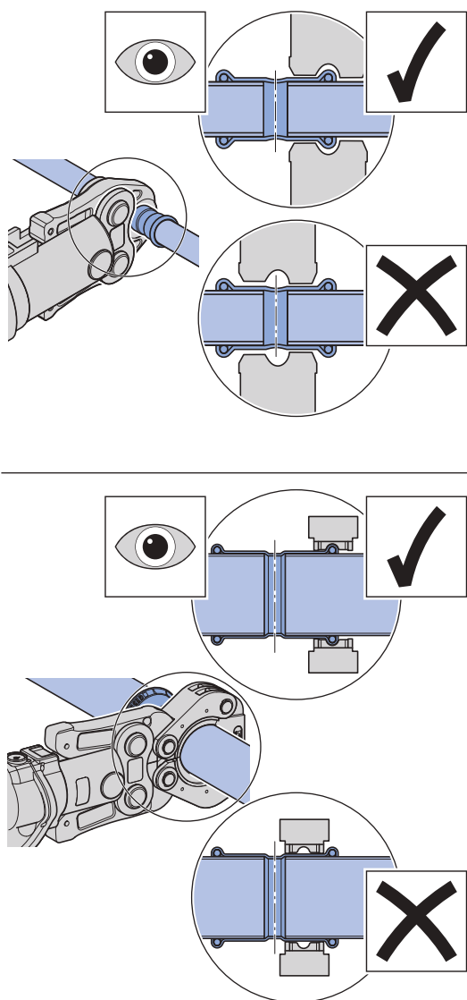
Figure 207: Positioning of the Geberit Mapress pressing jaw and pressing collar
