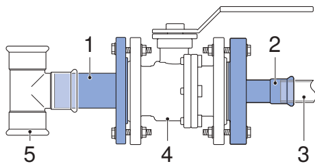
Figure 74: Connection to flange valves
