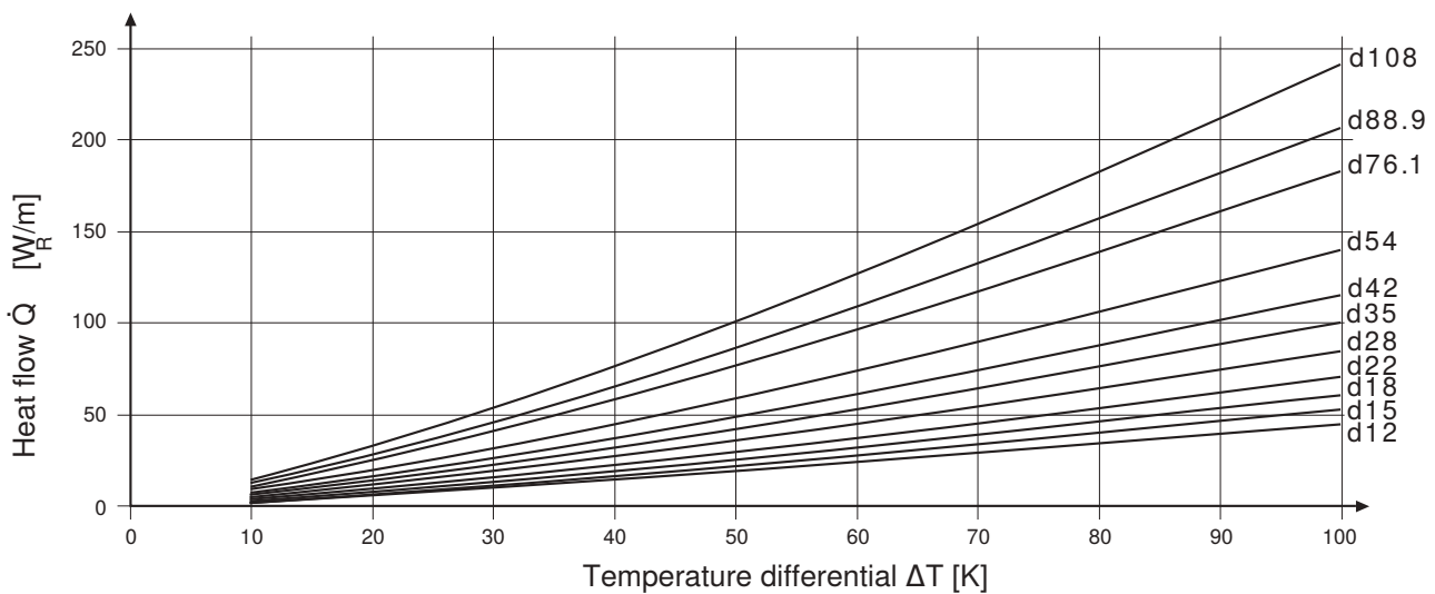
Figure 213: Heat emissions for copper pipes
