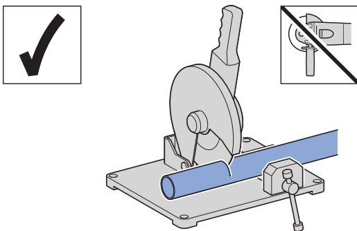
Figure 199: Suitable cutting tool
