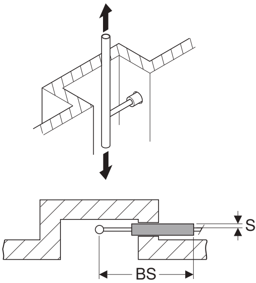
Figure 154: Straight deflection leg, with insulation
