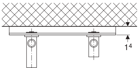
Figure 198: Installation dimension for exposed installation with a Geberit mounting plate, straight
