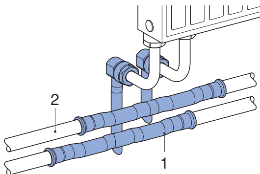
Figure 132: Skirting board connection with adapter with union connector for Euro cone
