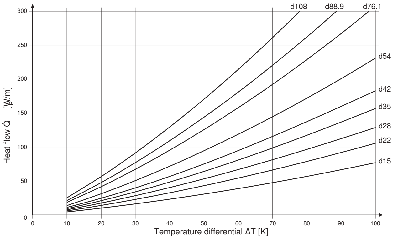
Figure 214: Heat emission for Geberit Mapress CuNiFe system pipes
