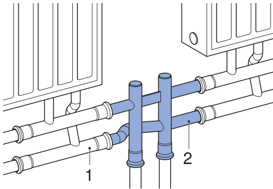
Figure 77: Connection to end piece for riser pipe
