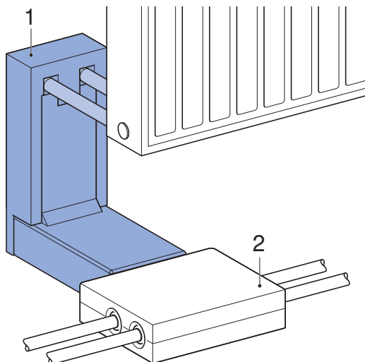
Figure 134: Radiator connector box type C for higher screed constructions
