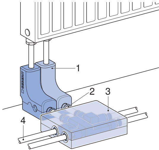
Figure 127: Radiator connection for pipe laying with a distance to the wall
