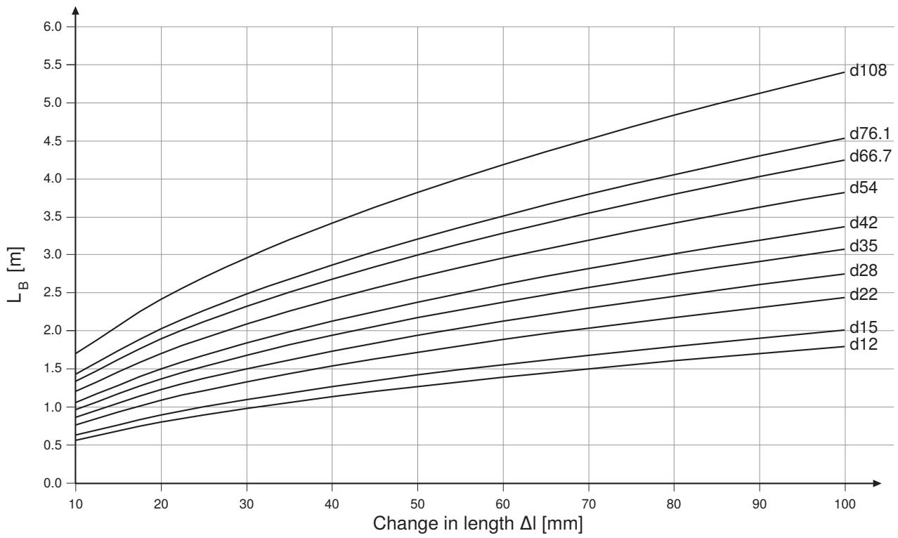
Figure 172: Deflection leg length L_B , copper pipes according to EN 1057
