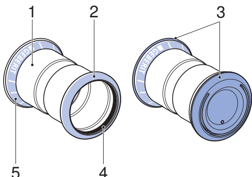
Figure 3: Structure of the Geberit Mapress threaded socket
