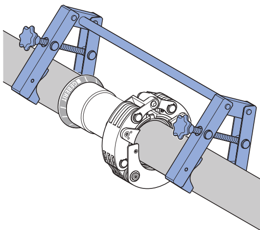
Figure 206: Geberit Mapress mounting aid MH1
