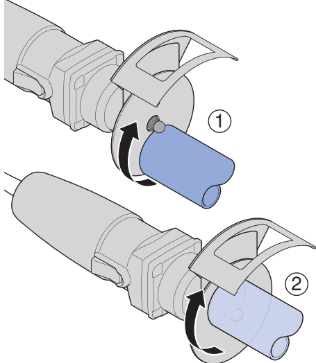
Figure 202: Deburring with a manual deburrer or with an electric pipe deburrer
