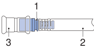
Figure 111: Connection to Geberit Mepla
