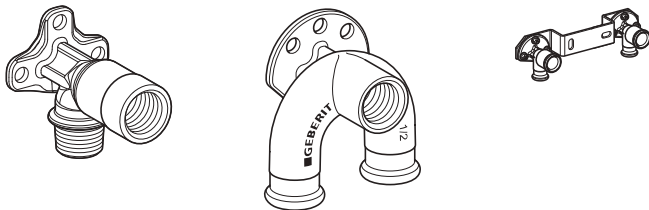
Figure 96: Geberit connections, stainless steel and gunmetal
