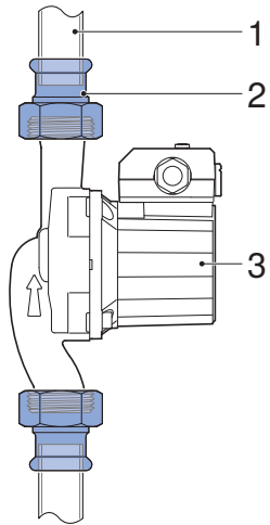
Figure 72: Connection to male thread
