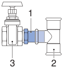
Figure 114: Connection to stop valve
