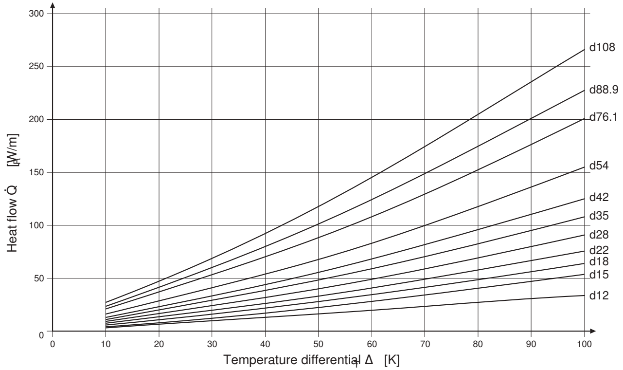
Figure 211: Heat emission for Geberit Mapress Stainless Steel 1.4401
