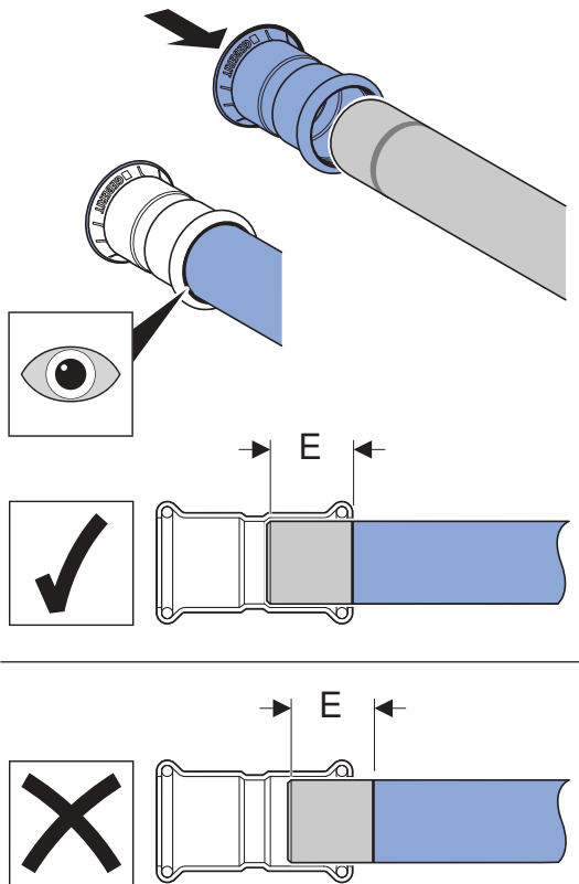
Figure 205: Marking on the pipe to check the correct insertion distance
