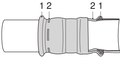
Figure 5: Pressed joint after pressing
